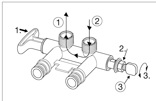
Fig. 37 Vanne bypass sur la position Bypass
